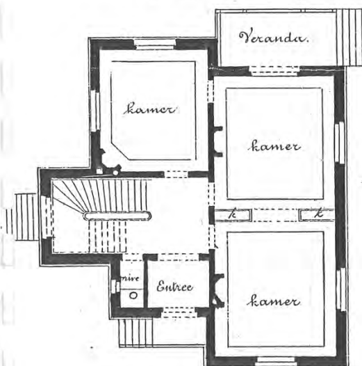
Benedenverdieping.
