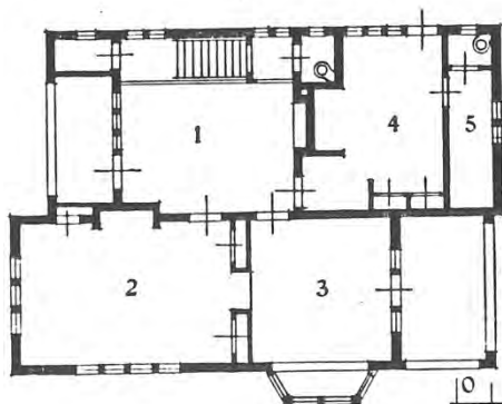
BEGANE GROND:
